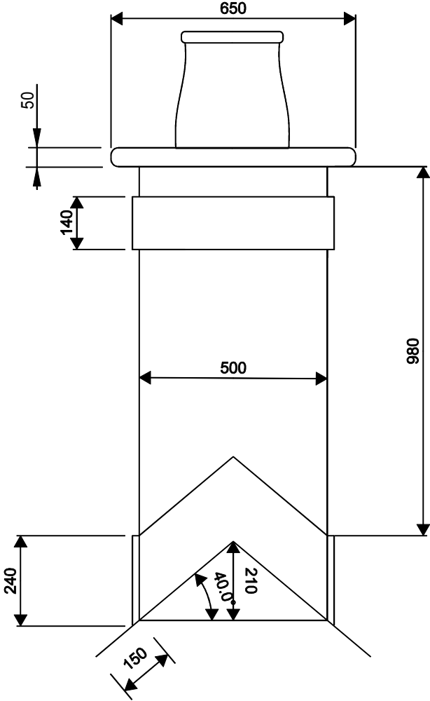
MID RIDGE SINGLE POT CHIMNEY 40 deg
