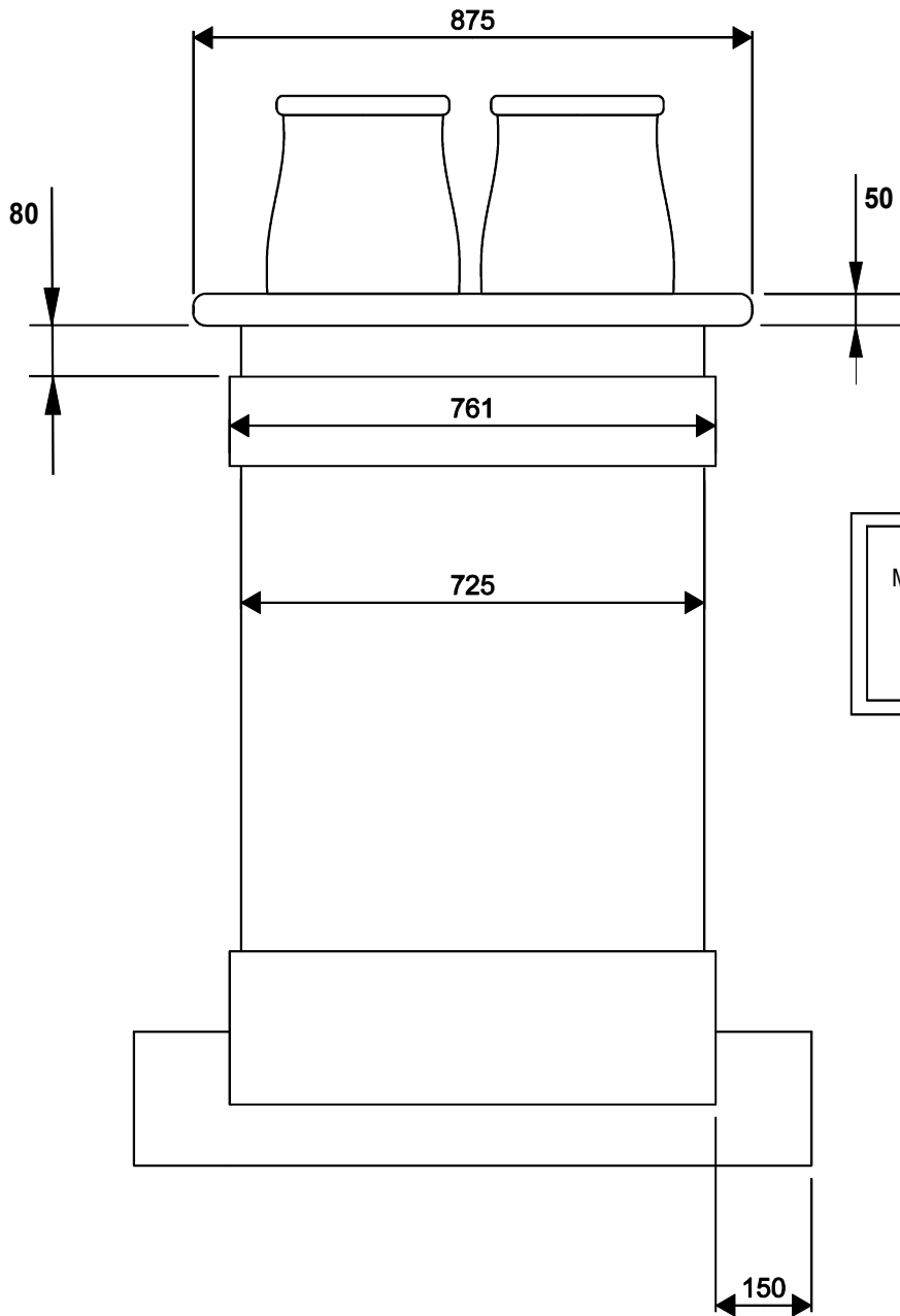
LONGITUDINAL MID RIDGE DOUBLE POT CHIMNEY
